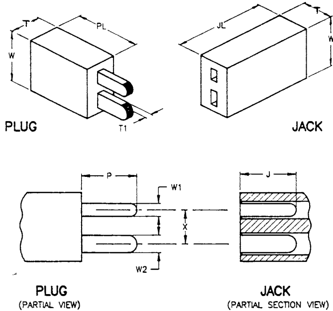
FIG. 1 Miniature Thermocouple Connector Dimensions (see Table 1 2)
