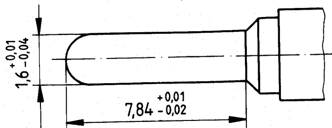
Figure 4 — Male contact
