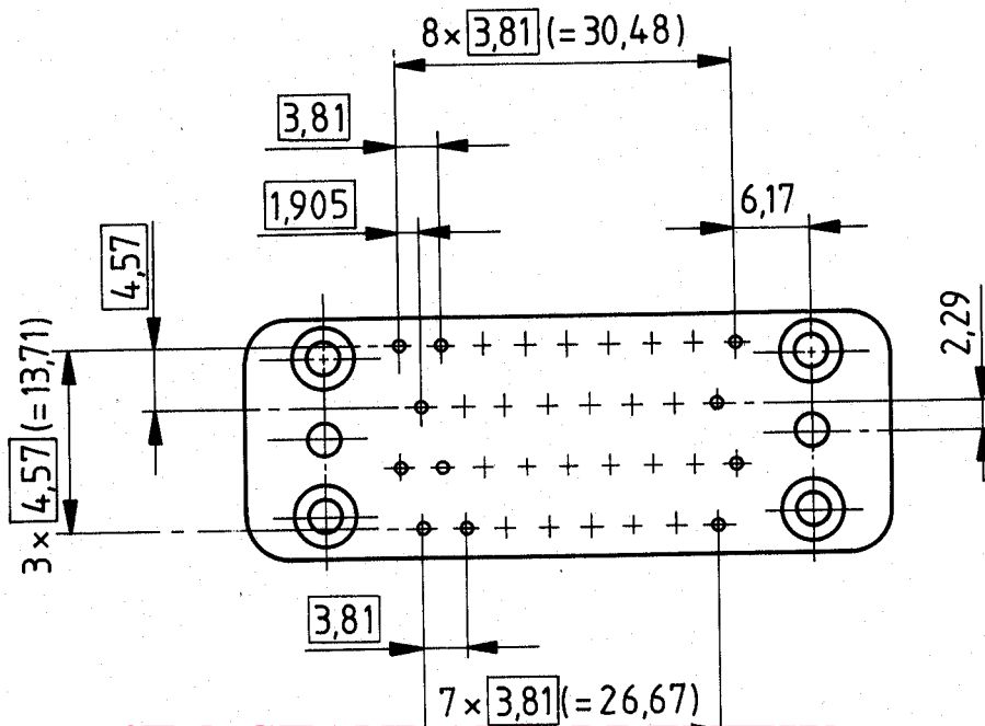
iTeh STANDARD PREVIEW (standards.iteh.ai) Figure 3 — Insert arrangement
