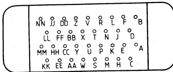
DTE connector face Contact identification lettering
