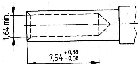
Figure 5 — Female contact
