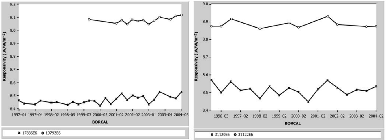
FIG. 1 Typical Within Laboratory Precision for Lab A (left) and Lab B (right) for Pyr heliometer Calibrations
