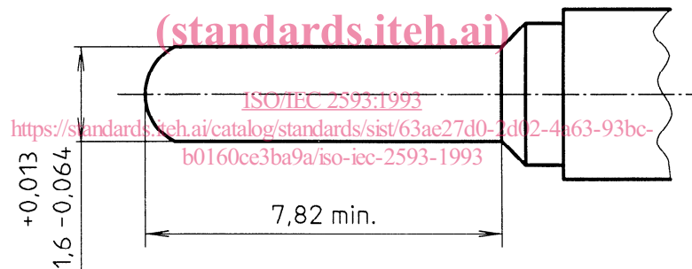
Figure 4 — Male contact
