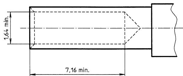
Figure 5 — Female contact
