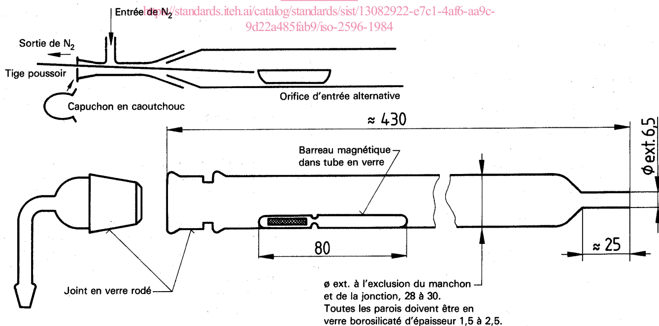
Figure 2 — Tube de dessiccation (5.3)
