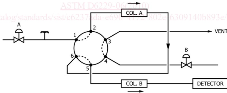
FIG. 1 Columns Connections to Switching Valve
