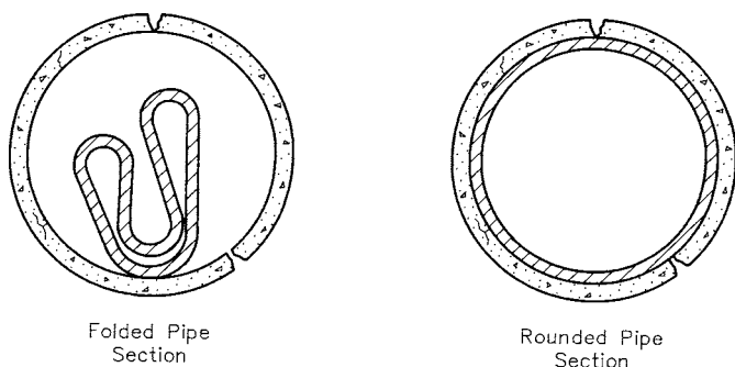
NOTE 1—This figure is intended only for clarification of terms specific to this specification and shows a representative folded pipe shape. Other folded pipe shapes may meet the requirements of this specification.
