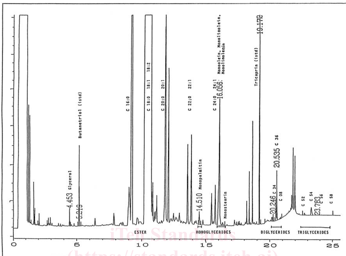
FIG. 1 Reference Chromatograms
