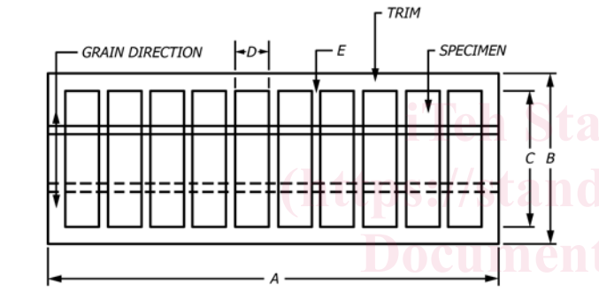
FIG. 3 Wood-to-Metal Tension Shear Test Specimen
