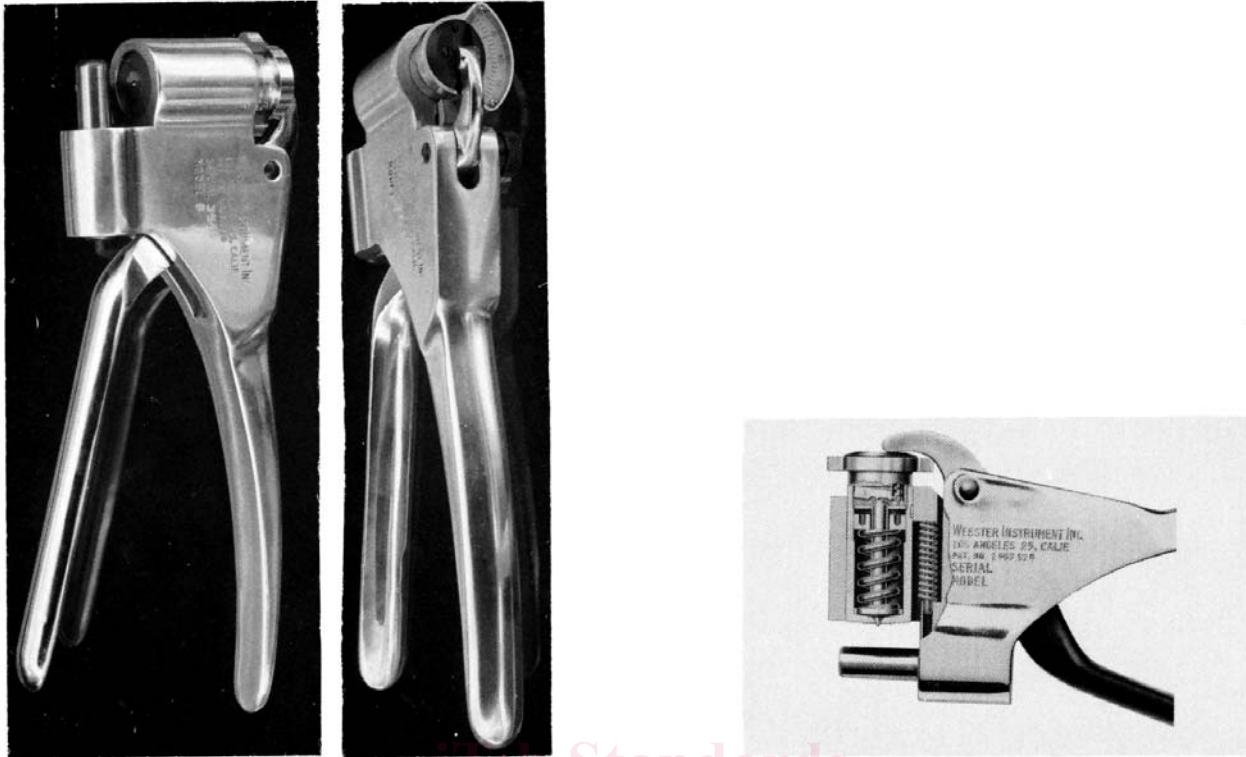
FIG. 1 Webster Hardness Gage, Model B
