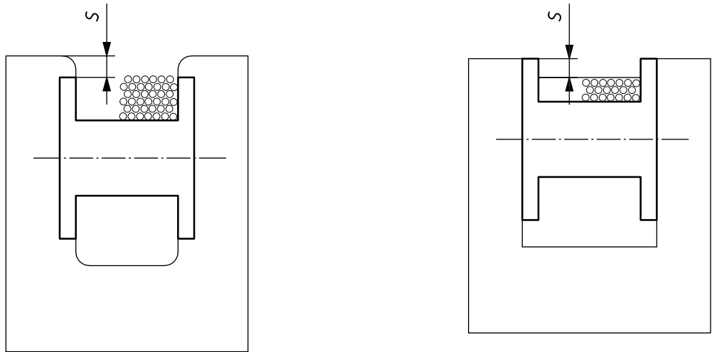
a) Winch with drum housing
