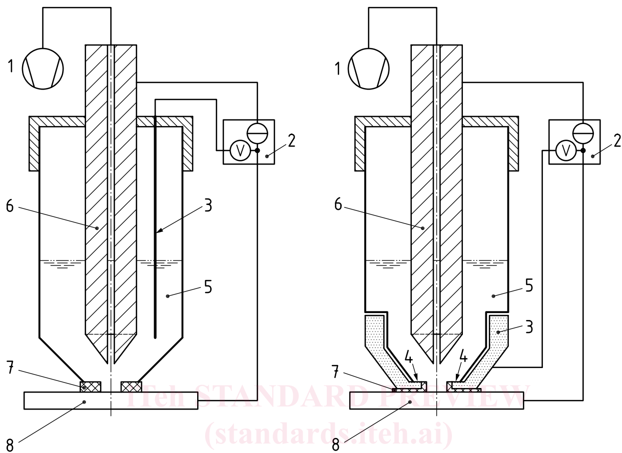
a) Measuring cell with silver wire, coated with AgCl, used as the reference electrode
