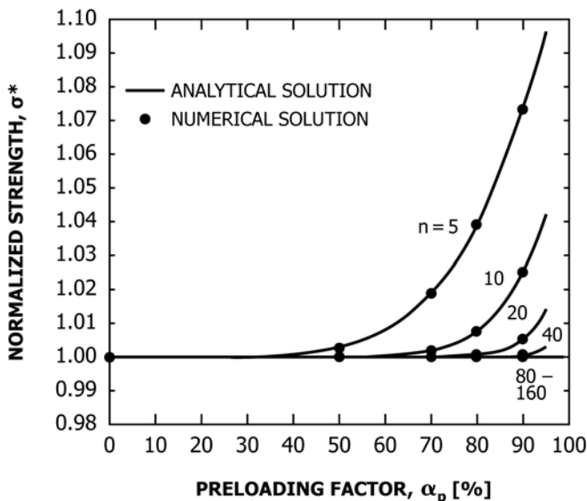
FIG. 1 Normalized Strength as a Function of Preloading for Different Slow Crack Growth Parameter n 's (Ref (12))
