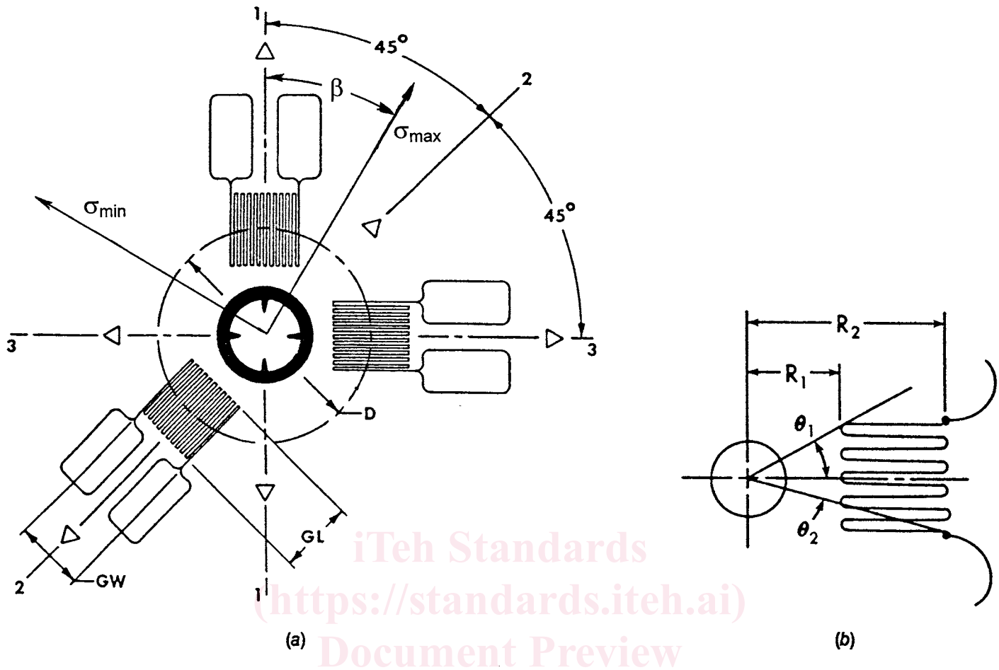
FIG. 1 Schematic Diagram Showing the Geometry of a Typical Three-Element Clockwise (CW) Strain Gage Rosette for the Hole-Drilling Method
