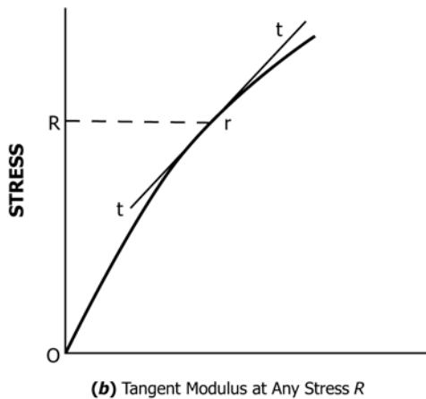
FIG. 1 Stress-Strain Diagrams Showing Straight Lines Corresponding to (a) Young’s Modulus, (b) Tangent Modulus, and (c) Chord Modulus
