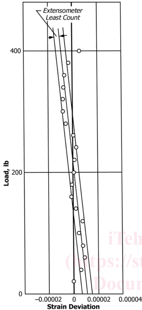
FIG. 2 Load-Deviation Graph
