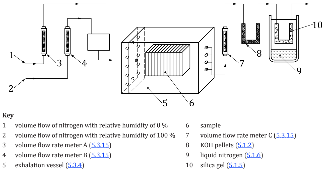
Figure 2 — Schematic representation of test bench
