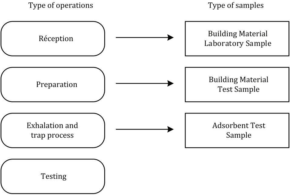
Figure 3 — Steps of measuring process with correspondent samples prepared
