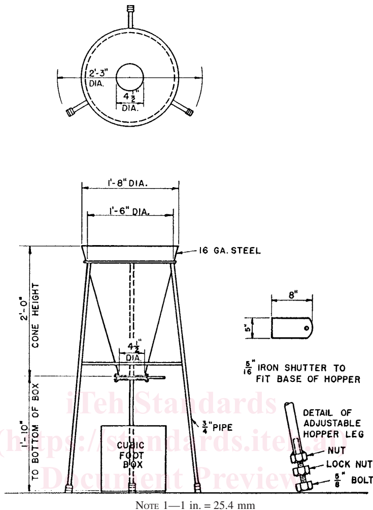
FIG. 1 Apparatus for Cone Procedure
