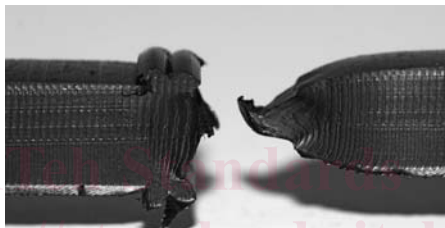
FIG. 3 Ductile Rupture Adjacent to Fusion Interface
