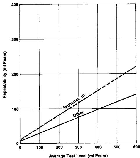
FIG. 3 Precision Chart—Repeatability
