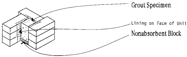
FIG. 1 Grout Mold (Units 6 in. (152.4 mm) or Less in Height, 2¼ in. (57.2 mm) High Brick Shown)
