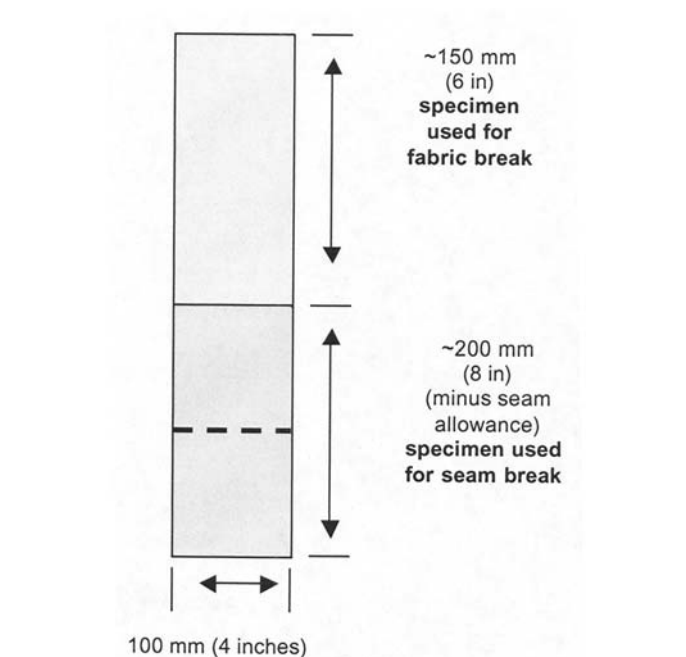
FIG. 1 Seamed Specimen Removed from Manufactured Item
