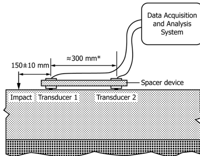
FIG. 2 Schematic of Testing Configuration for Procedure A
