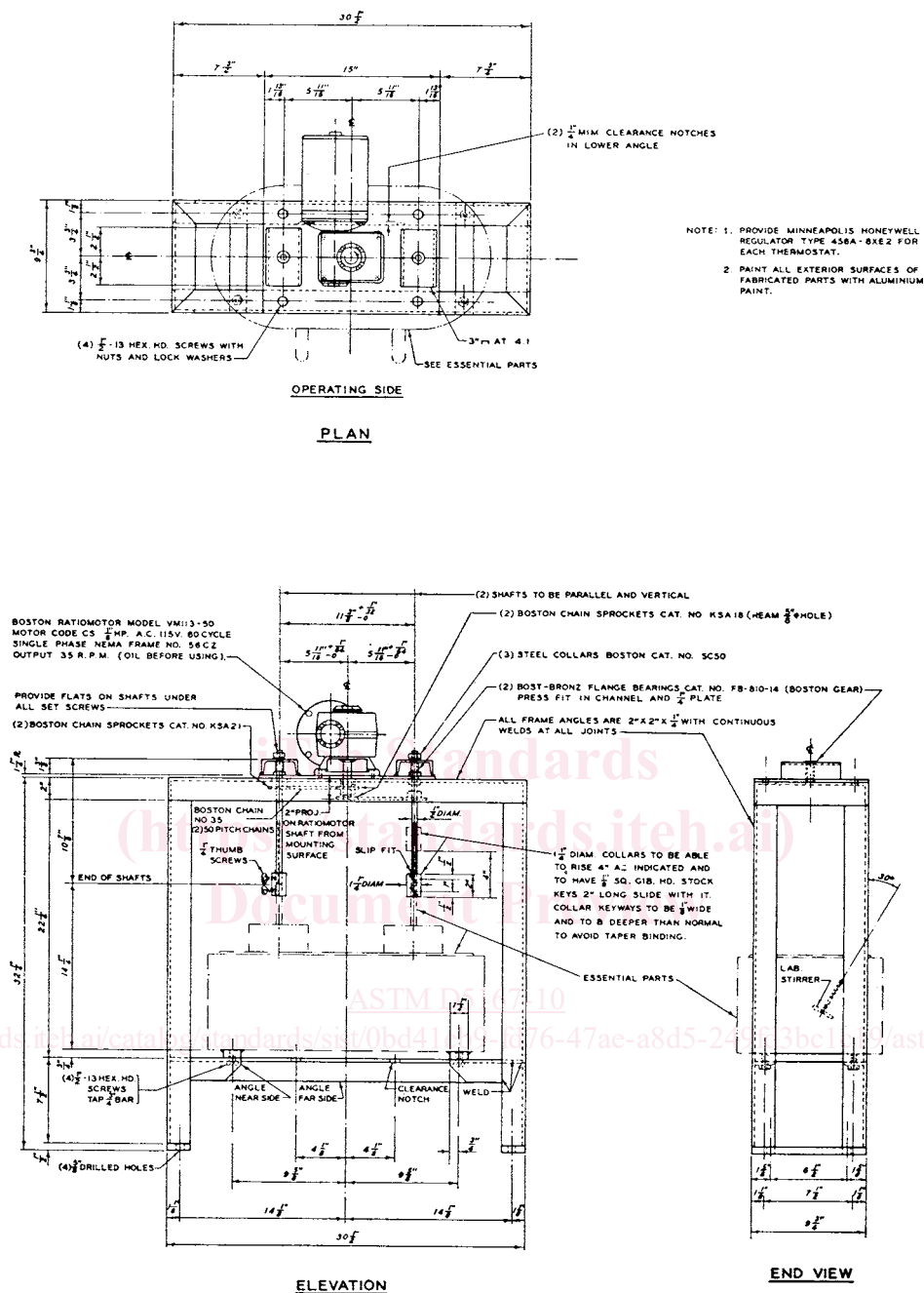
DRIVE AND FRAME FIG. 1 Detailed Drawing of Joint Sealant Laboratory Melting Unit
