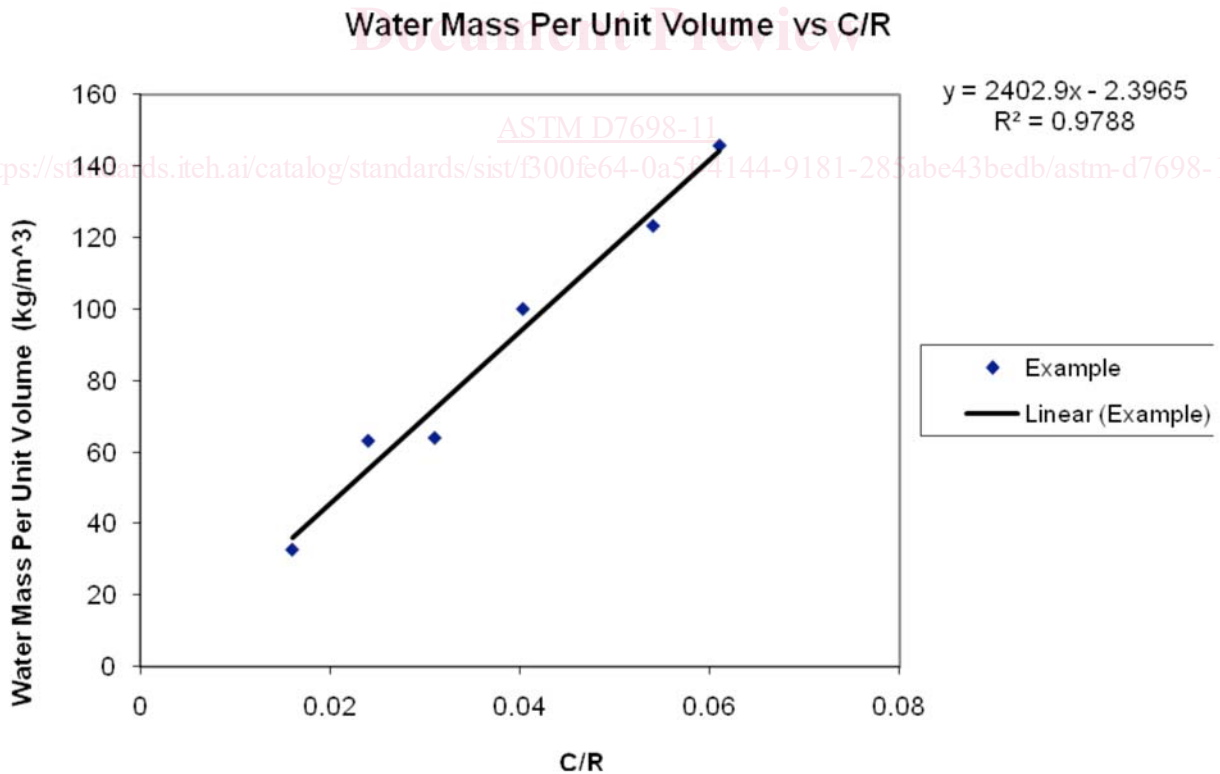
FIG. 3 Typical Values of Water Mass Per Unit Volume Vs. C/R (Regression Equation Upper Right)
