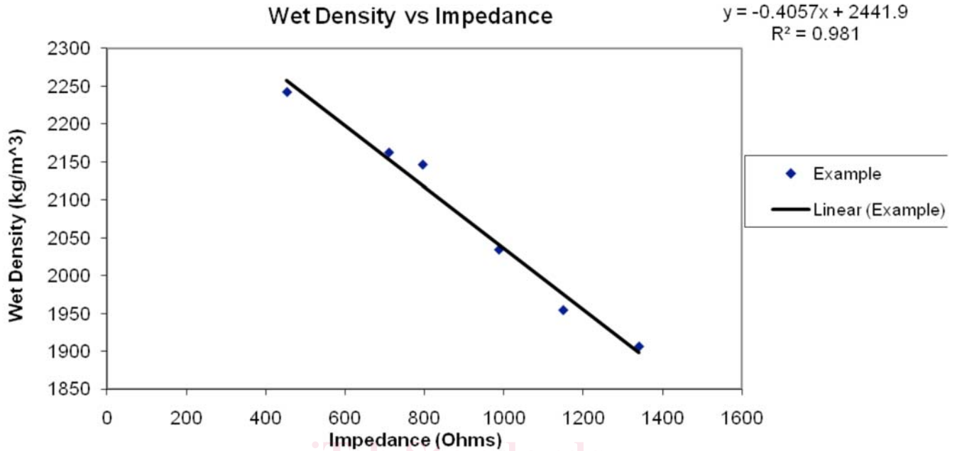
FIG. 2 Typical Values of Wet Density Vs. Impedance (Regression Equation Upper Right)
