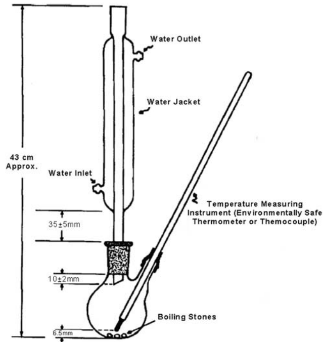
FIG. 1 Boiling Point Test Apparatus
