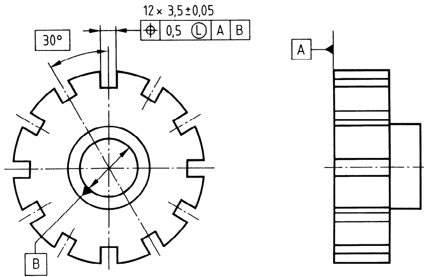
a) Indication on the drawing
