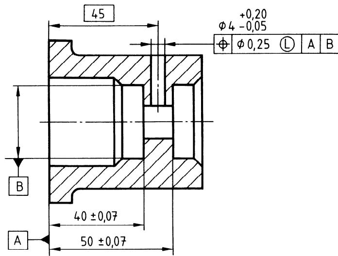
a) Indication on the drawing
