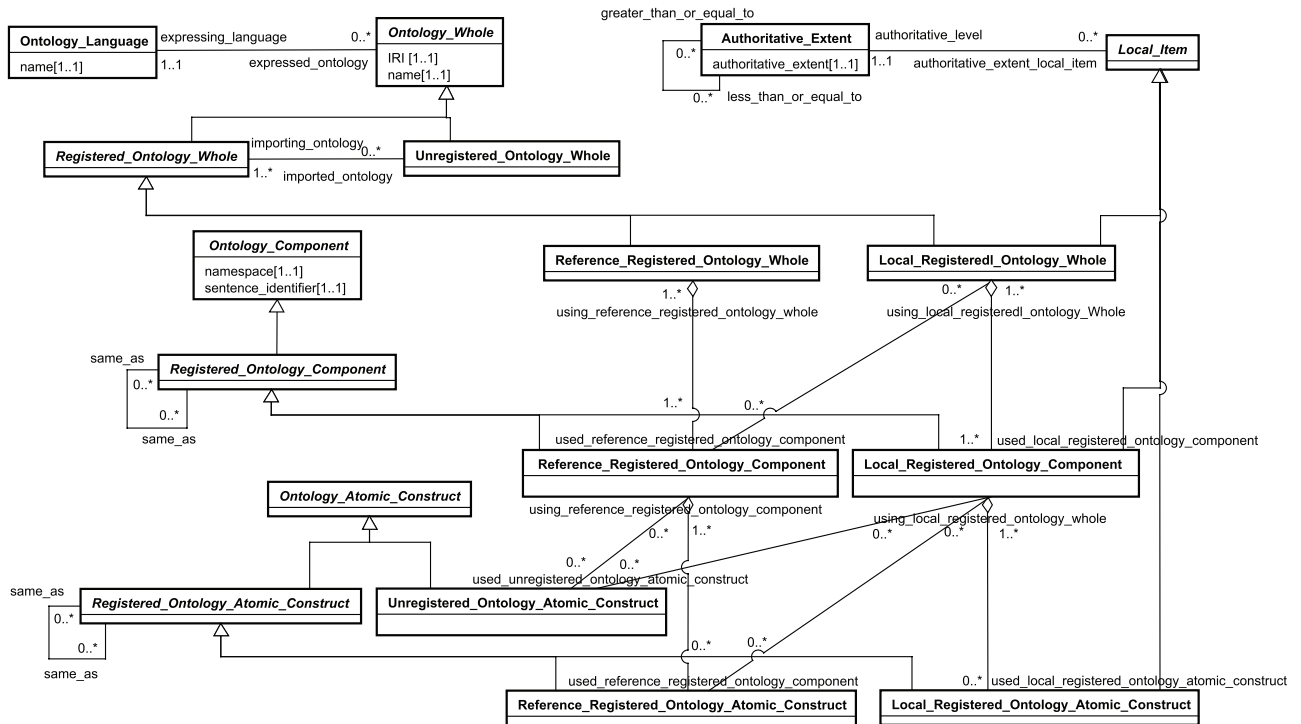
Figure 3 — Metamodel in Basic Model package (standards.iteh.ai)
