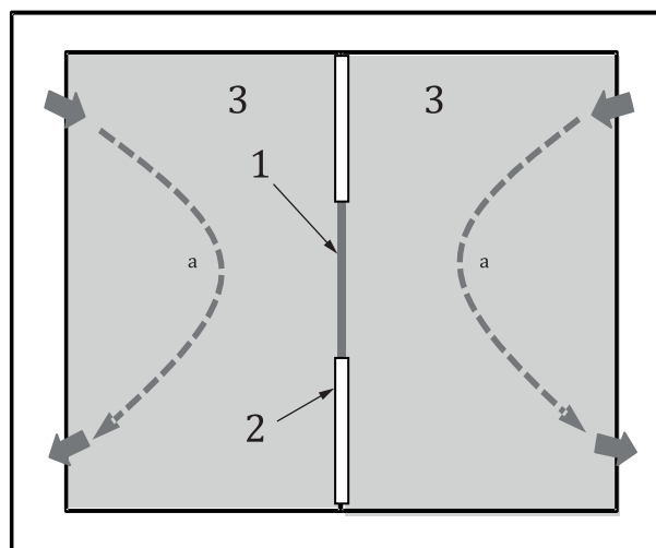
b) Temperature chamber having two rooms
