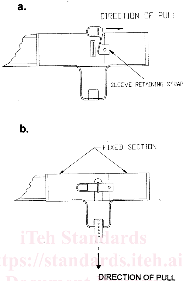
FIG. 9 a & b Sleeve Retaining Straps on Velcro Wrap Style Pads
