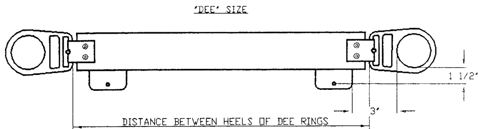
FIG. 10 “Dee” Measurement
