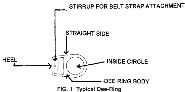
FIG. 1 Typical Dee-Ring
