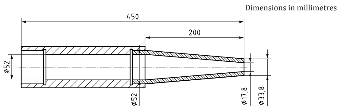
Figure 3 — Nozzle
