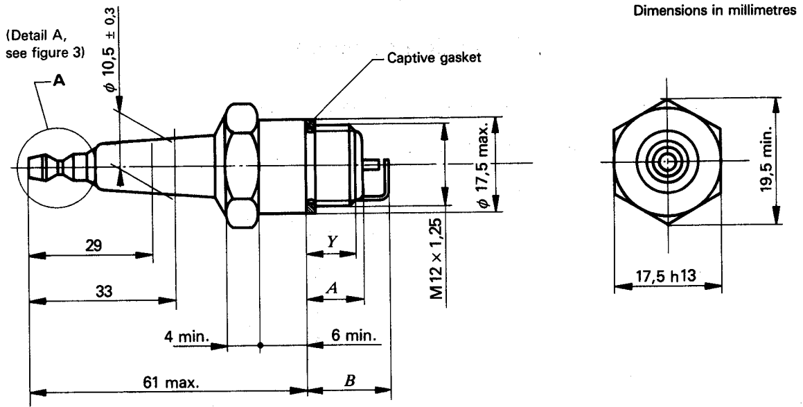
Figure 1 – Spark plug M 12 × 1,25 with flat seating
