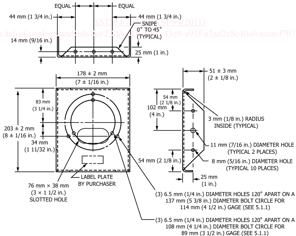
FIG. 1 Gauge Board Type I
