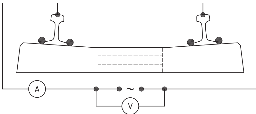
Figure 2 — Measurement circuit
