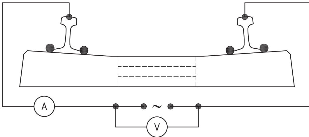
Figure 2 — Measurement circuit
