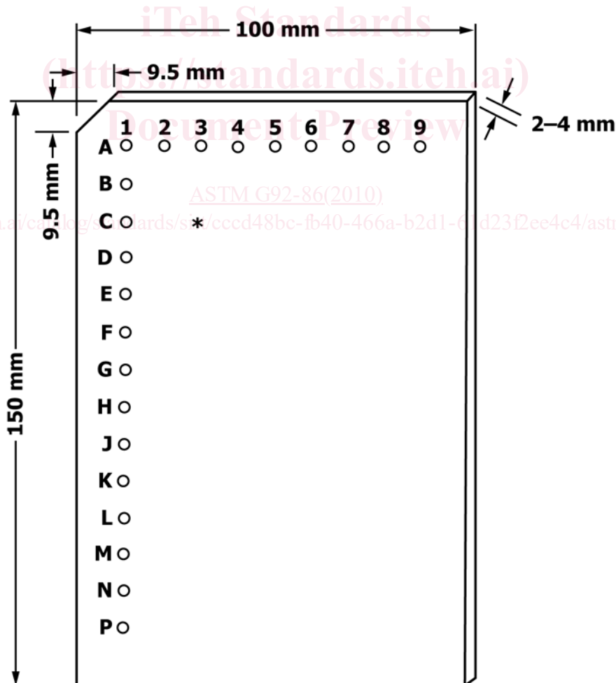
FIG. 1 Sample Atmospheric Specimen Drill Code Identification Template
