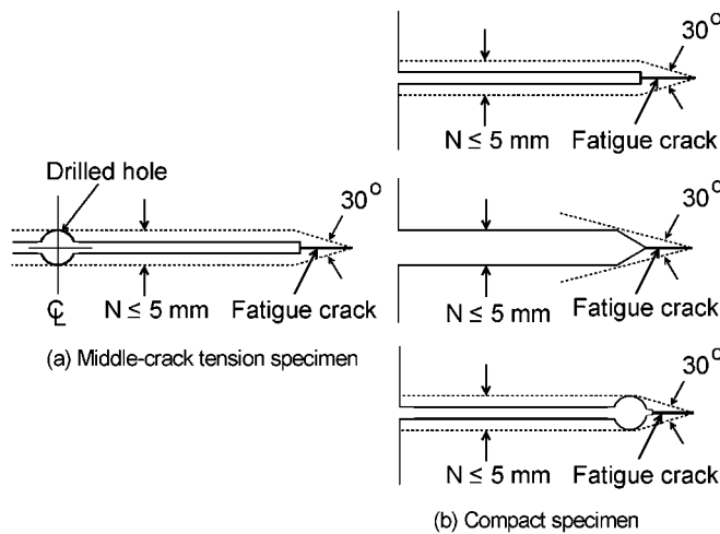
FIG. 7 Envelope of Fatigue Crack Starter Notch Configurations
