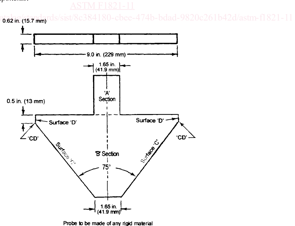
FIG. 4 Test Probe for Partially Bounded Openings
