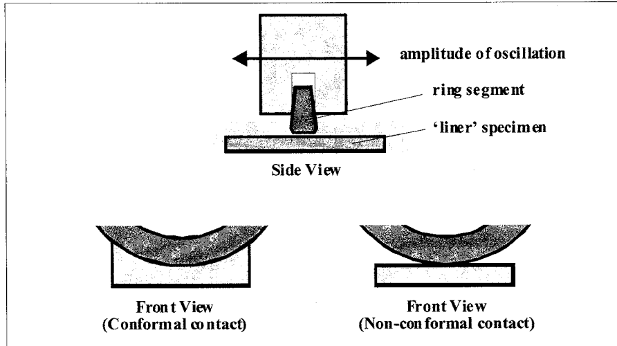
FIG. 1 Schematic Drawing of the Test Configuration Showing Conformal and Non-conformal Contact
