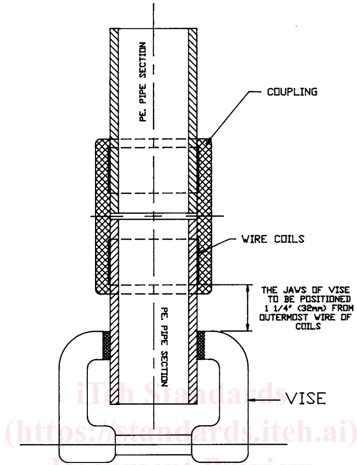
FIG. 2 Coupling Crush Test Arrangement
