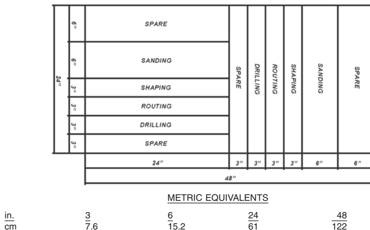
FIG. 2 Diagram for Sawing Wood-Base Panel Samples into Smaller Samples for Individual Tests
