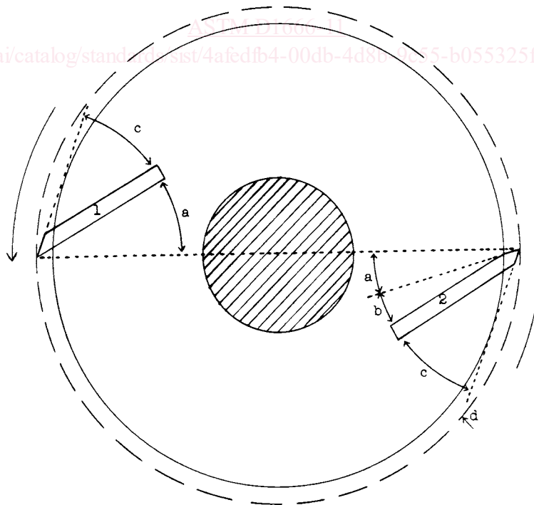
FIG.-4 5 Terms Used in Connection with Planer Knives
