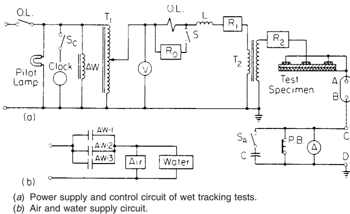
FIG. 3 Circuit Diagrams
