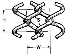
FIG. 1 Mesh Dimensions for 5/8-in., 1/2-in., and 3/8-in. Fabric
