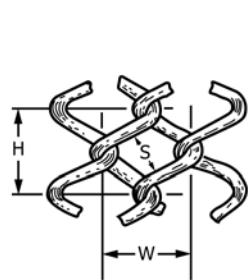
FIG. 1 Mesh Dimensions for 5/8-in., 1/2-in., and 3/8-in. Fabric
