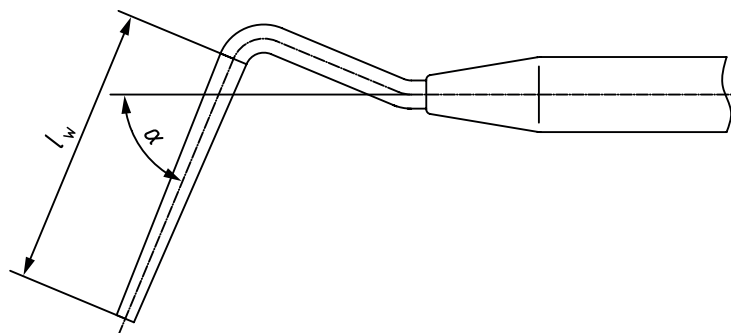
Figure 3 — Binangle compactor
