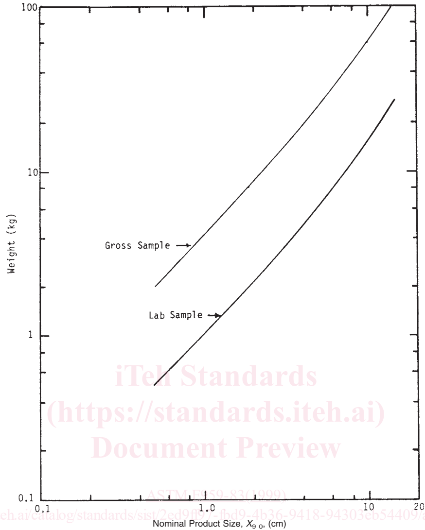
FIG. 3 Weight Requirements for Gross and Lab Samples as a Function of Nominal Product Size
