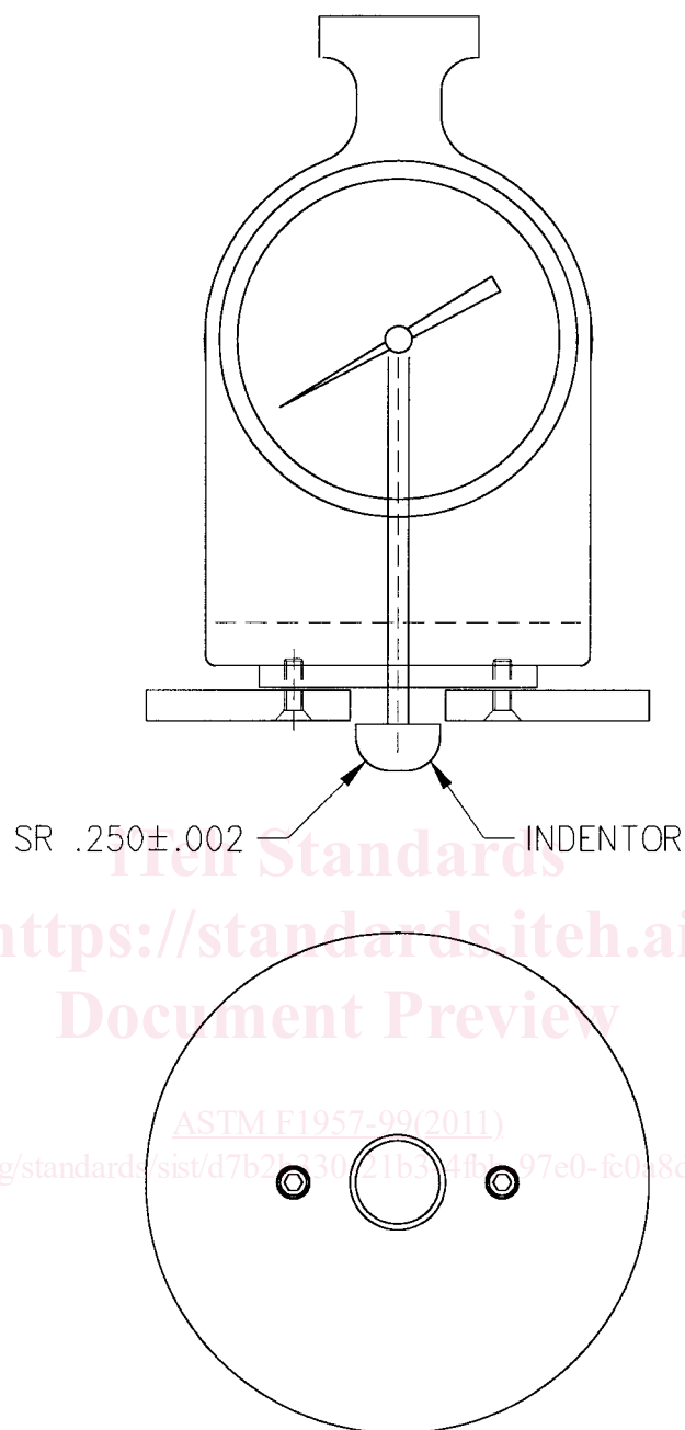
FIG. 2 Indentor Detail
