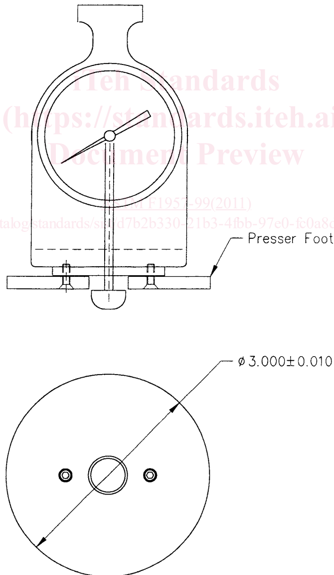
FIG. 1 Presser Foot Detail
