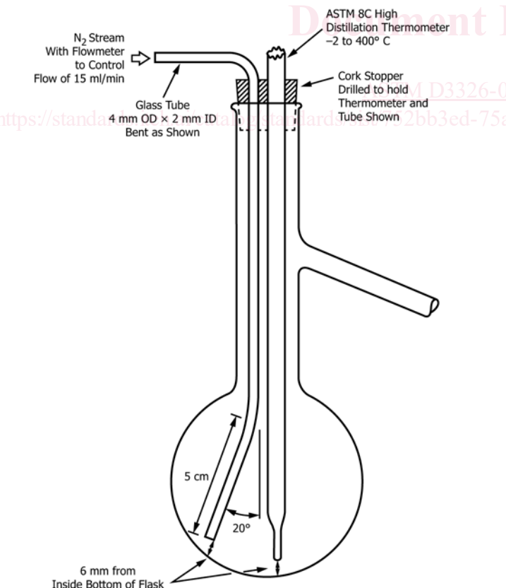
FIG. 1 Adaptation of ASTM Distillation Flask for Topping Chloroform Solutions of Oil to Simulate Weathering
