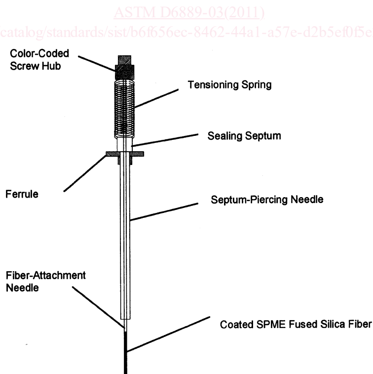
FIG. 1 Fiber Holder
