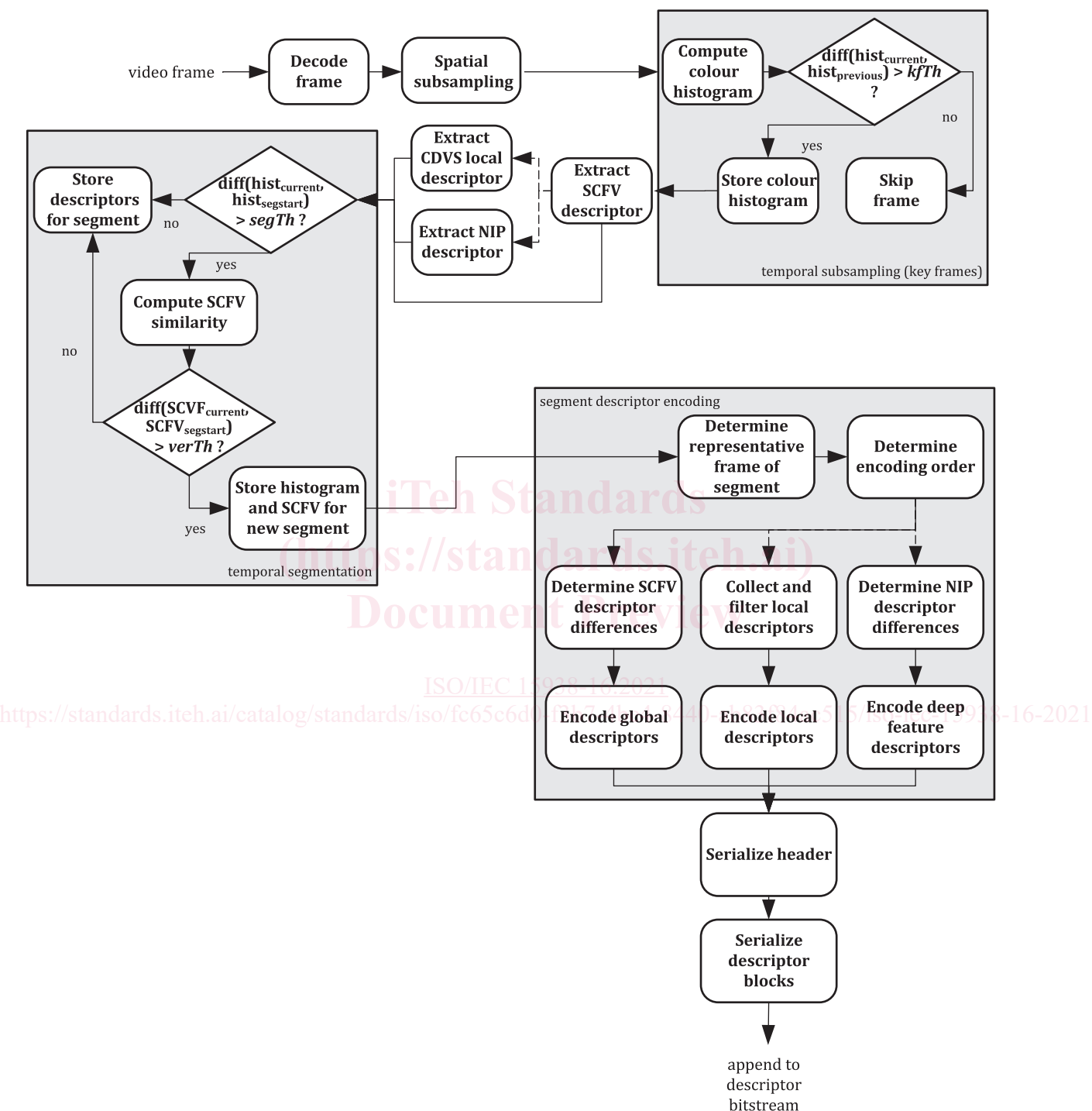
Figure 1 — CDVA descriptor extractor
