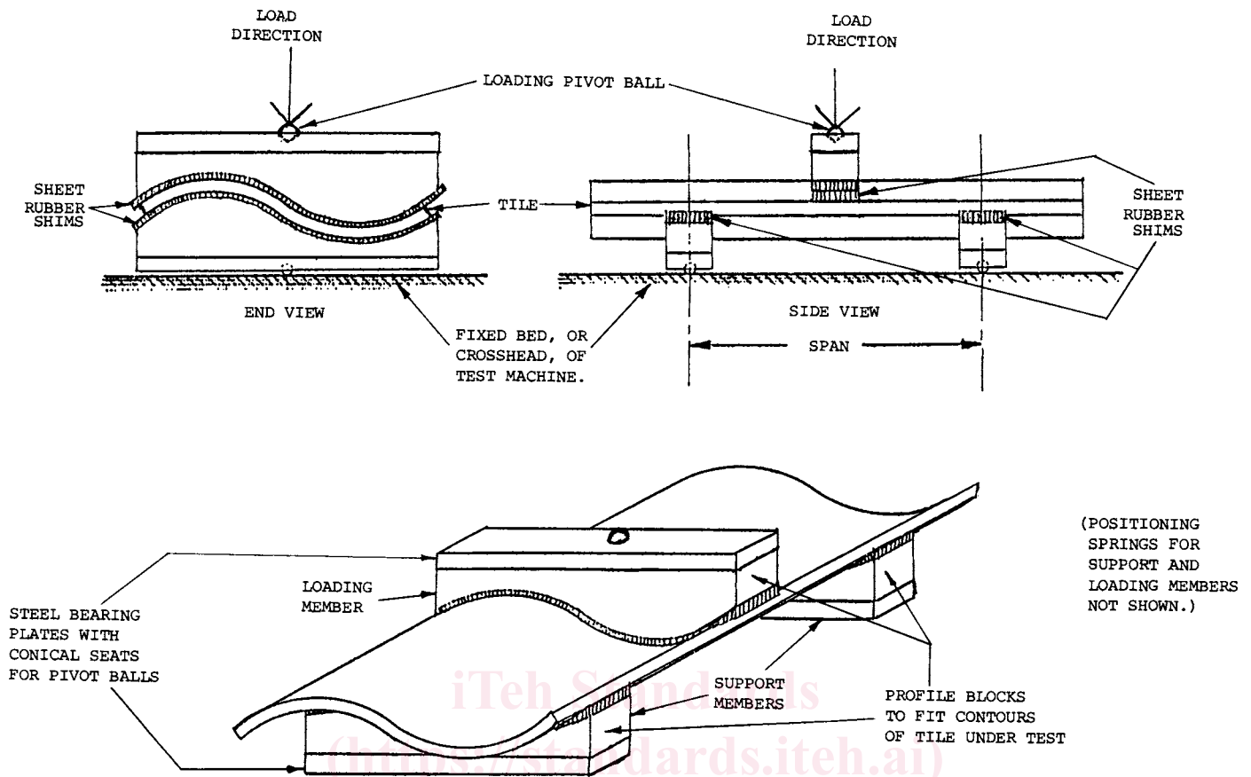
FIG. 1 Schematic of Assembly for Flexure Strength Testing
